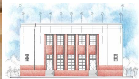
SOUTH ELEVATION SEE OTHER
